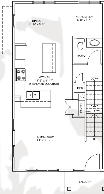
MAIN (WITH STANDARD KITCHEN LOCATION) 626 SQ. FT
